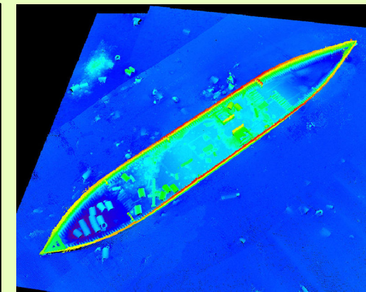
Multibeam data collected on an underwater wreck found in the Gulf of Mexico
